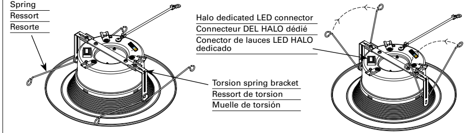
Figure 7. LED Connection
