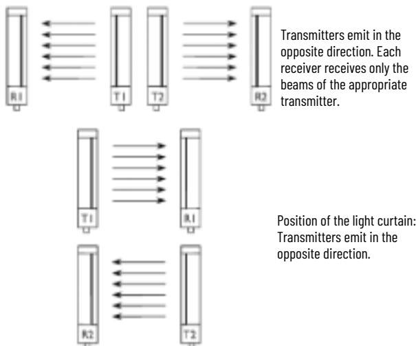
Figure 6 - Multiple Unit Alignment Options
