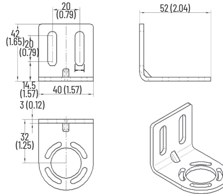
Figure 7 - Mounting Brackets [mm (in.)]
