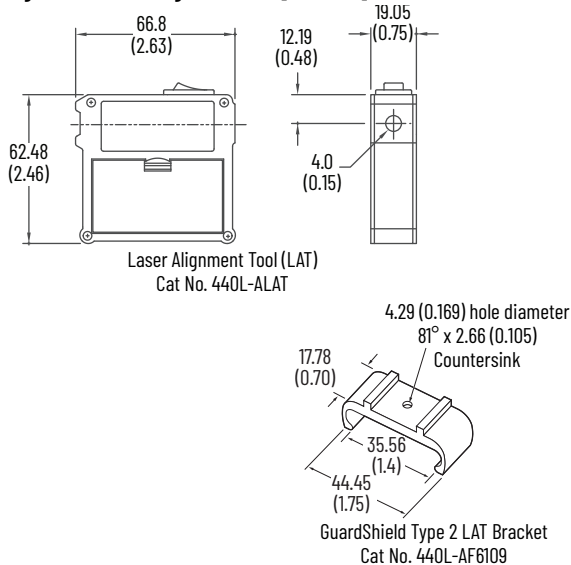
Figure 19 - Laser Alignment Tool [mm (in.)]
