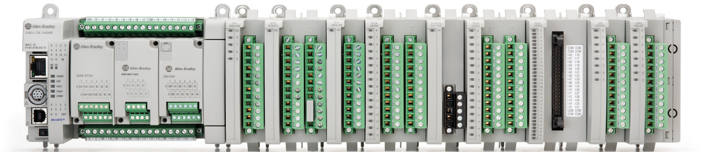
A Micro870 controller with plug-in modules, eight expansion I/O modules, and an expansion I/O power supply attached
